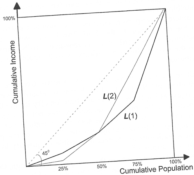
Figure 6.7. Ambiguous comparisons: A Lorenz crossing.
